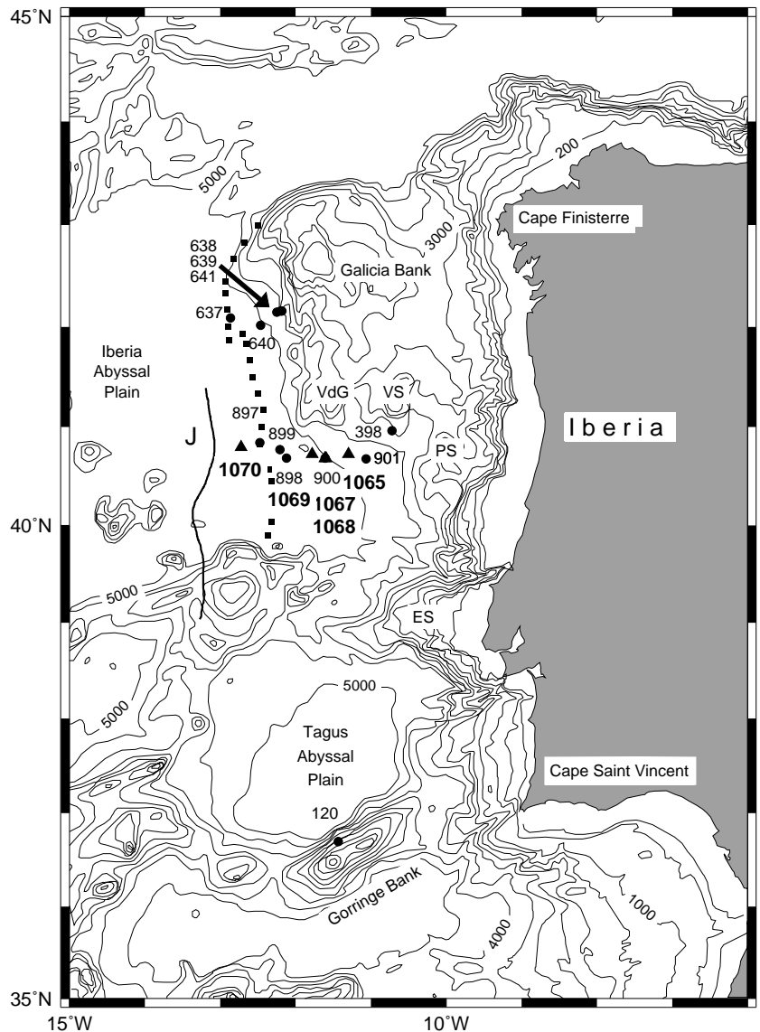
Figure 1. Bathymetric chart of the west Iberia margin showing the Leg 173 (triangles), and earlier (dots), drill sites. The small squares and the bold line mark the peridotite ridge and the J-anomaly, respectively.
