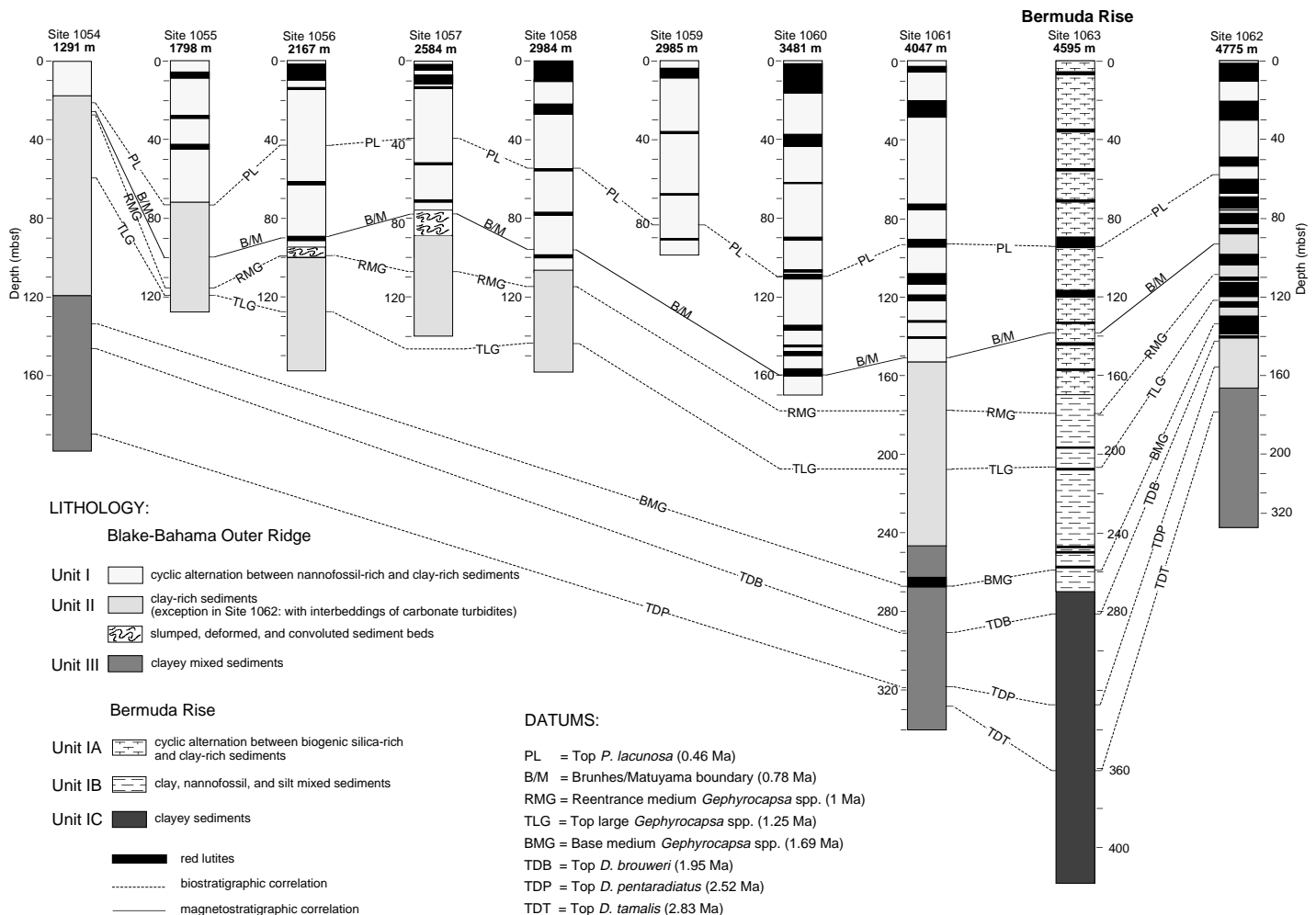
Figure 2. Summary of litho-, bio- and magnetostratigraphy for Leg 172 sites (excepting Sohm Abyssal Plain Site 1064). Sites 1054 through 1063 all contain similar lithologic units of similar ages, attesting to the strong and coherent control of western North Atlantic circulation patterns on sedimentation. Especially noteworthy is the occurrence of red lutites, which seem to be more prevalent in the late Pleistocene at deeper sites, and the curious occurrence of late Pleistocene biogenic silica-rich sediments on the Bermuda Rise.
