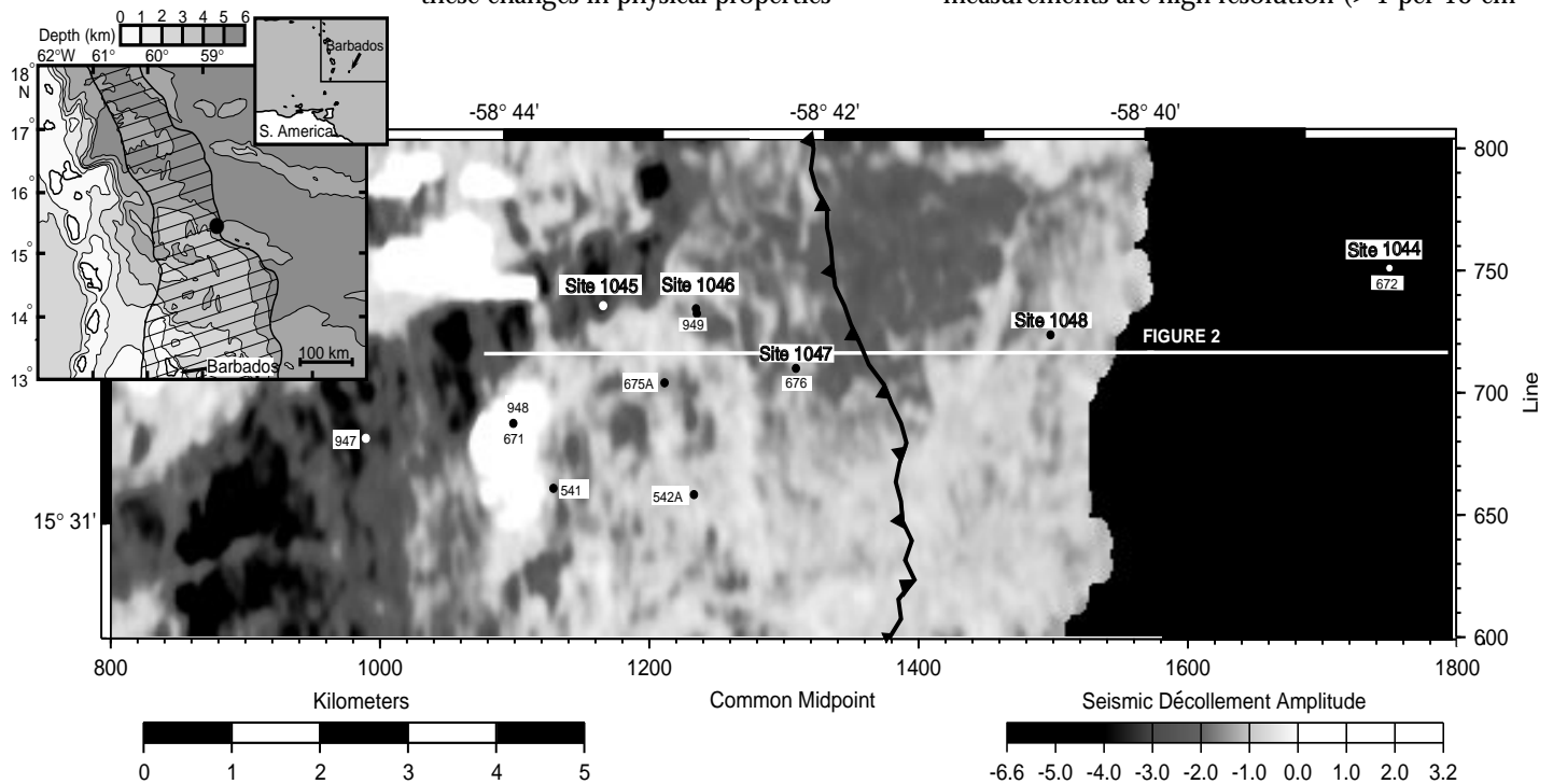
Figure 1. Location of ODP Leg 171A area, Barbados accretionary prism. Sites are shown over a map of peak seismic reflection amplitude of décollement zone and part of proto-décollement zone (after Shipley et al., 1994 and Moore et al., 1995). Line shows location of cross section shown in Figure 2.
