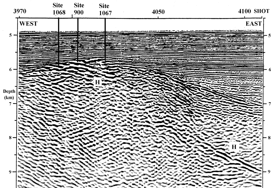
Figure 2. Part of multi-channel seismic reflection profile Lusigal-12 that has been pre-stack depth migrated by Krawczyk et al. (1996) (no vertical exaggeration). The figure shows the relative locations of Sites 1067, 1068 and 900 over Hobby High. H marks two possibly unconnected, but strong, intrabasement reflectors (see text).
