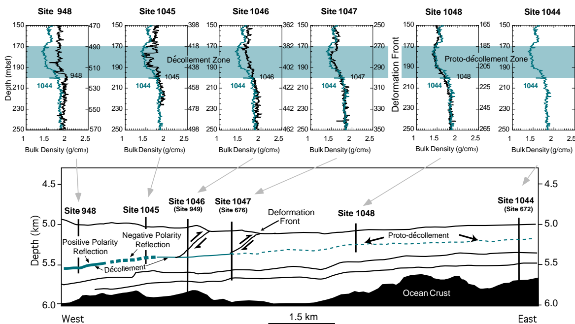
Figure 2. Generalized cross section showing LWD density distribution through proto-décollement zone or décollement zone at all sites. Depth scale on left side of density plots refers to depth of Site 1044 data; depth scale on right side of density plots refers to depth scale for the site indicated by the arrow. Horizontal bar shows approximate depth of proto-décollement and décollement zones across all sites. Site 1044 LWD data are used to represent the baseline undeformed reference density pattern.
